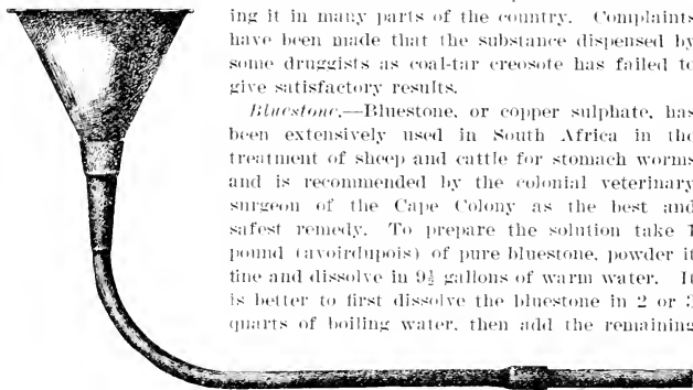
FIG. 21.—A drenching tube made from an ordinary tin funnel, a piece of rubber hose, and a piece of brass pipe.
